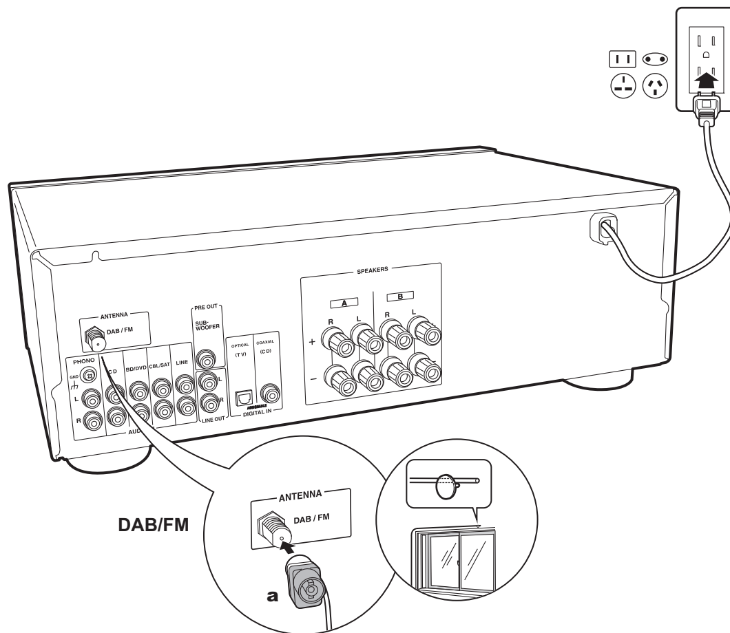
a FM/DAB-antenn
